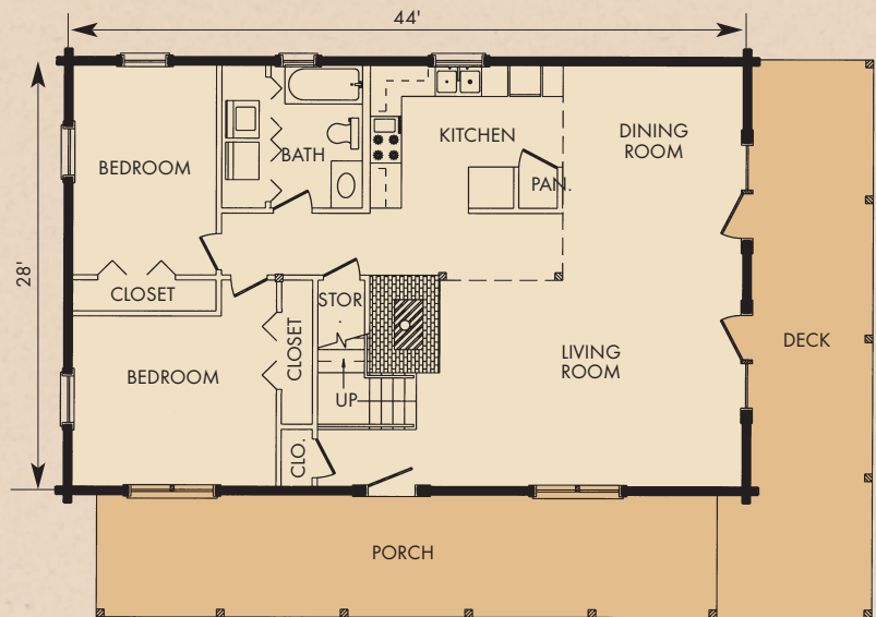
MAIN FLOOR
